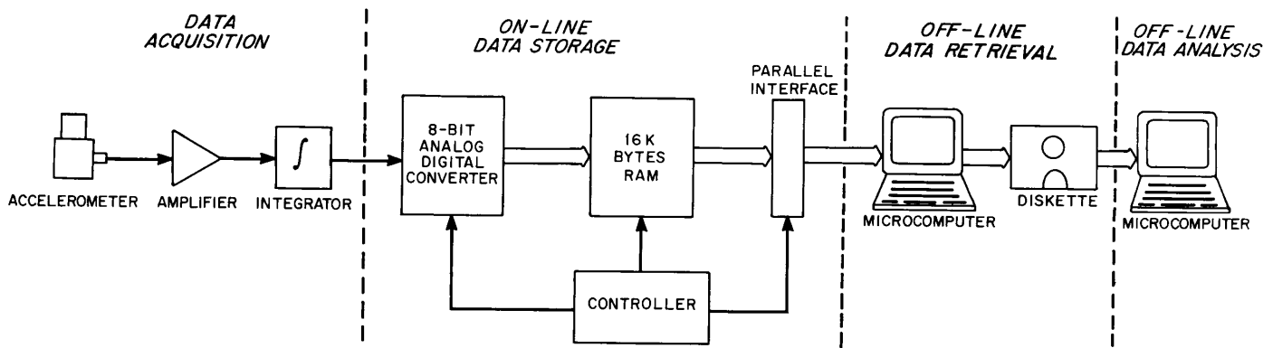
Figure 2—Block diagram of vibration exposure assessment scheme. Tool operation is sampled using an accelerometer attached to the hand tool, the acceleration waveform amplified, integrated, digitized, and stored in RAM on-line. Off-line the data is retrieved using a portable microcomputer and stored on diskette for later analysis.
