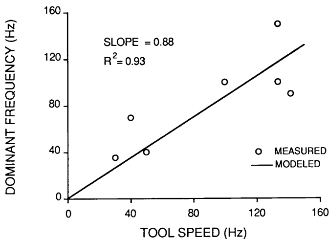
Figure 5—Plot of rotary and reciprocating tool dominant fundamental frequencies versus rated tool free running speed (n=7).
