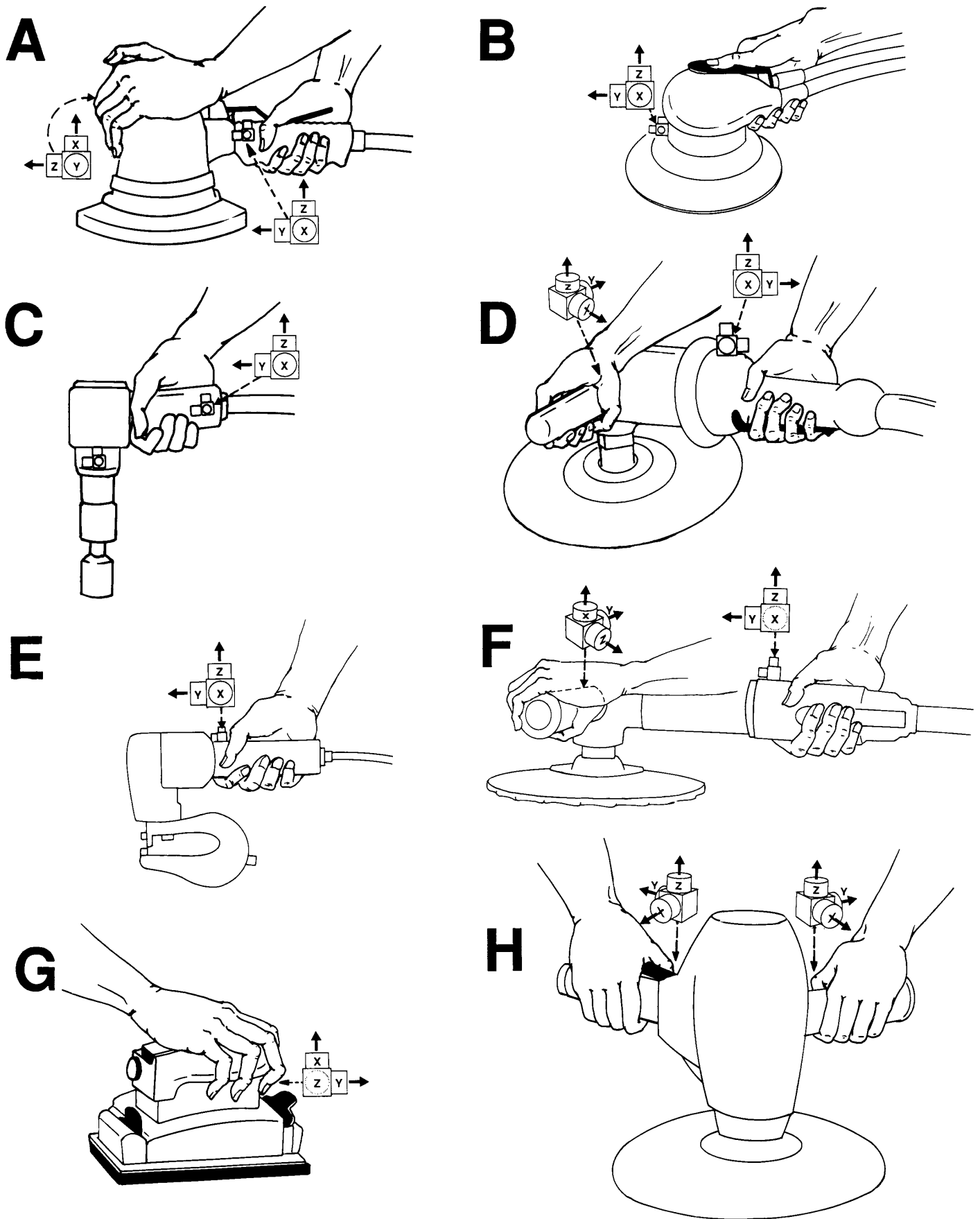
Figure 1—Handle and grip posture for the eight tools included in the survey. Accelerometer locations and corresponding coordinates in the x, y, and z axes are also included. (A) Hand grip orbital sander, (B) Palm grip orbital sander, (C) Impact wrench, (D) Heavy duty right angle sander, (E) Trimming shear, (F) Light duty right angle sander, (G) Jitterbug sander, (H) Vertical polisher.
